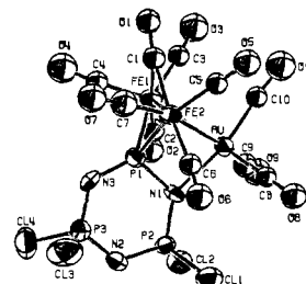
Figure 5. ORTEP diagram for compound 7 .
